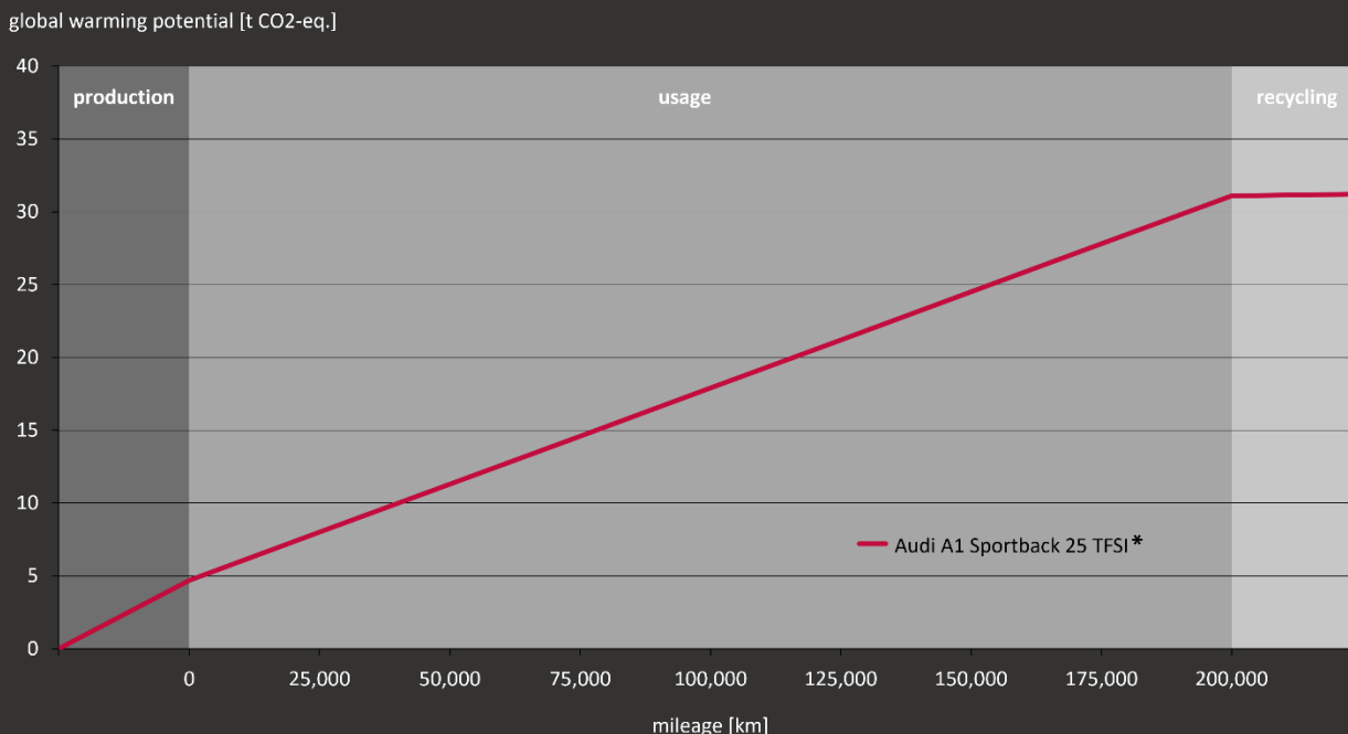
Figure 2: Global warming potential of the Audi A1 Sportback 25 TFSI* over the entire life cycle
