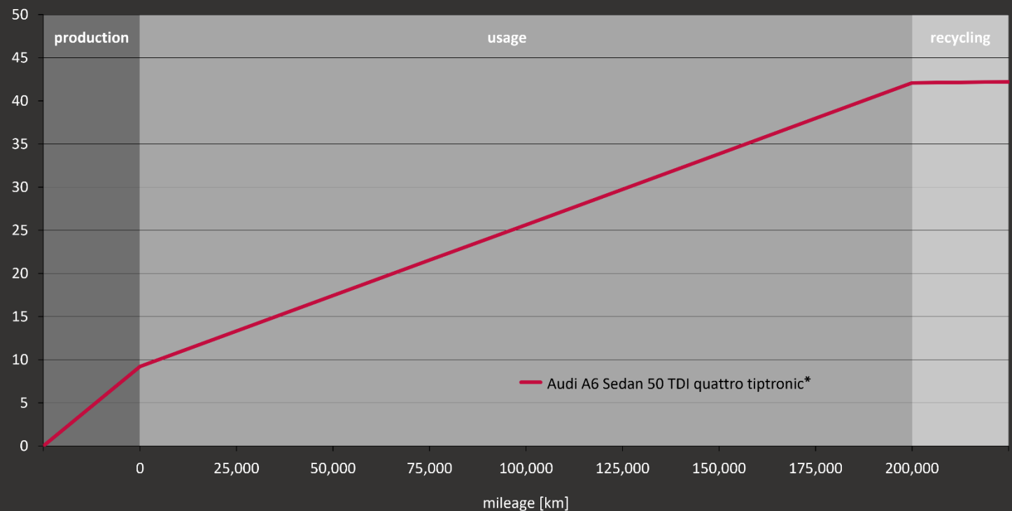
Figure 2: Global warming potential of the Audi A6 Sedan 50 TDI quattro tiptronic* over the entire life cycle
